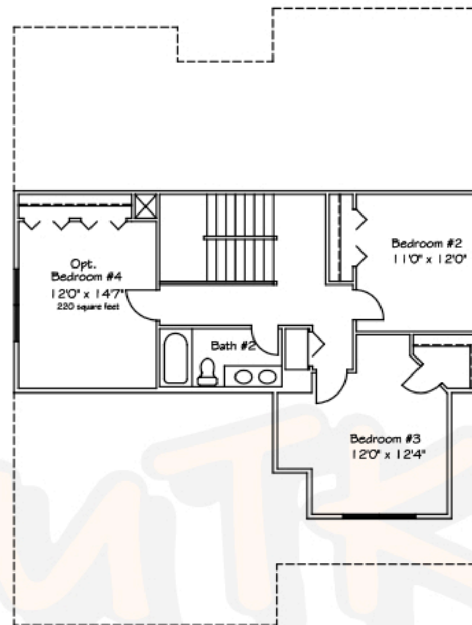
SECOND FLOOR
