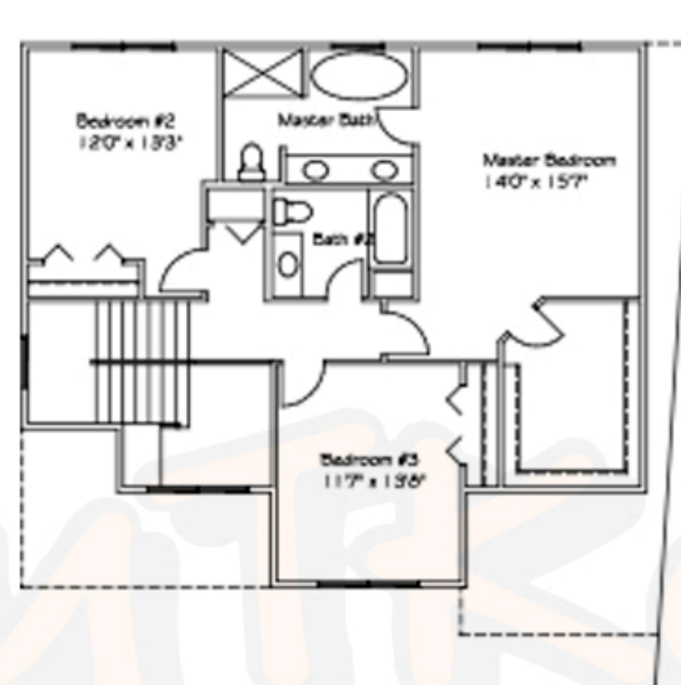
SECOND FLOOR
