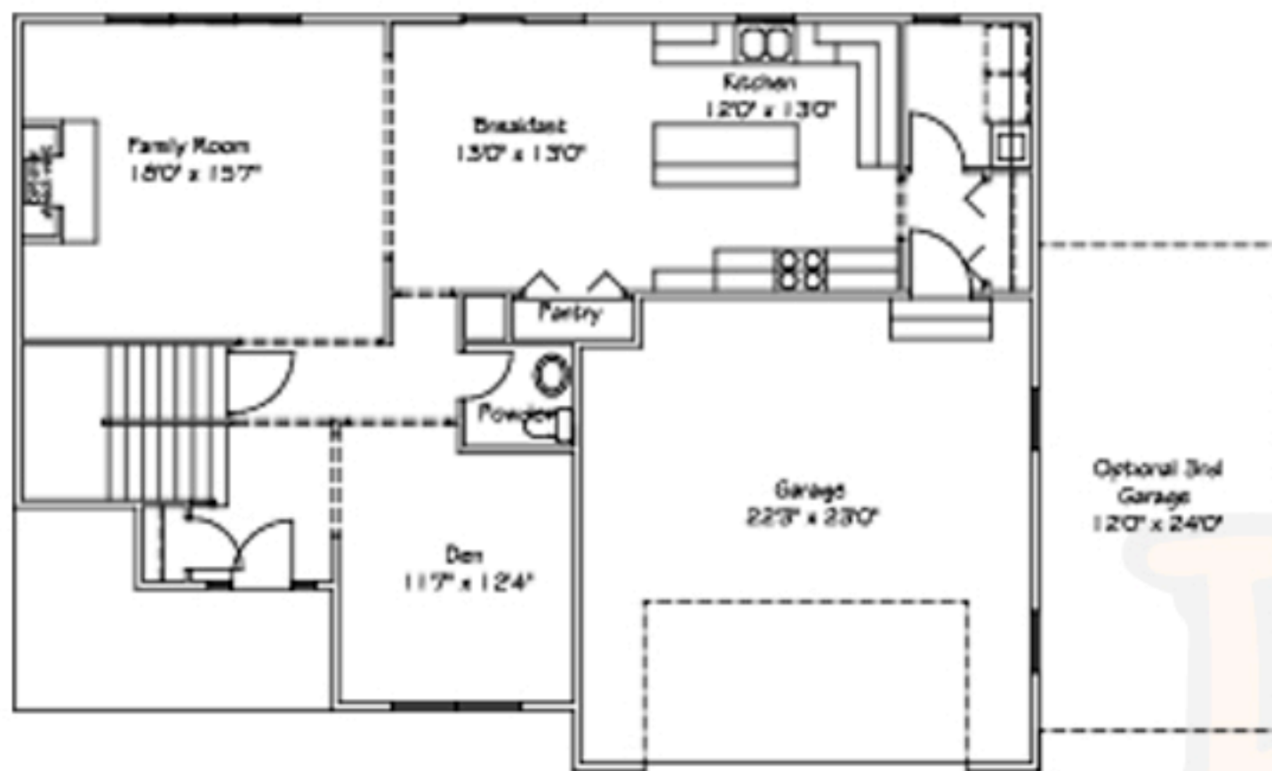
MAIN FLOOR
